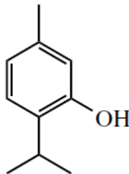
timol
