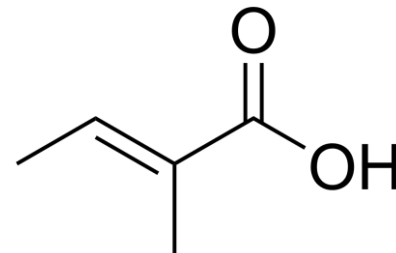
tiglinska kiselina
